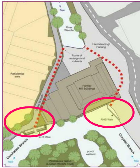
Figure 5.2 Option 2: Full Weir Removal with Pre-Barrages / Step-Pools
